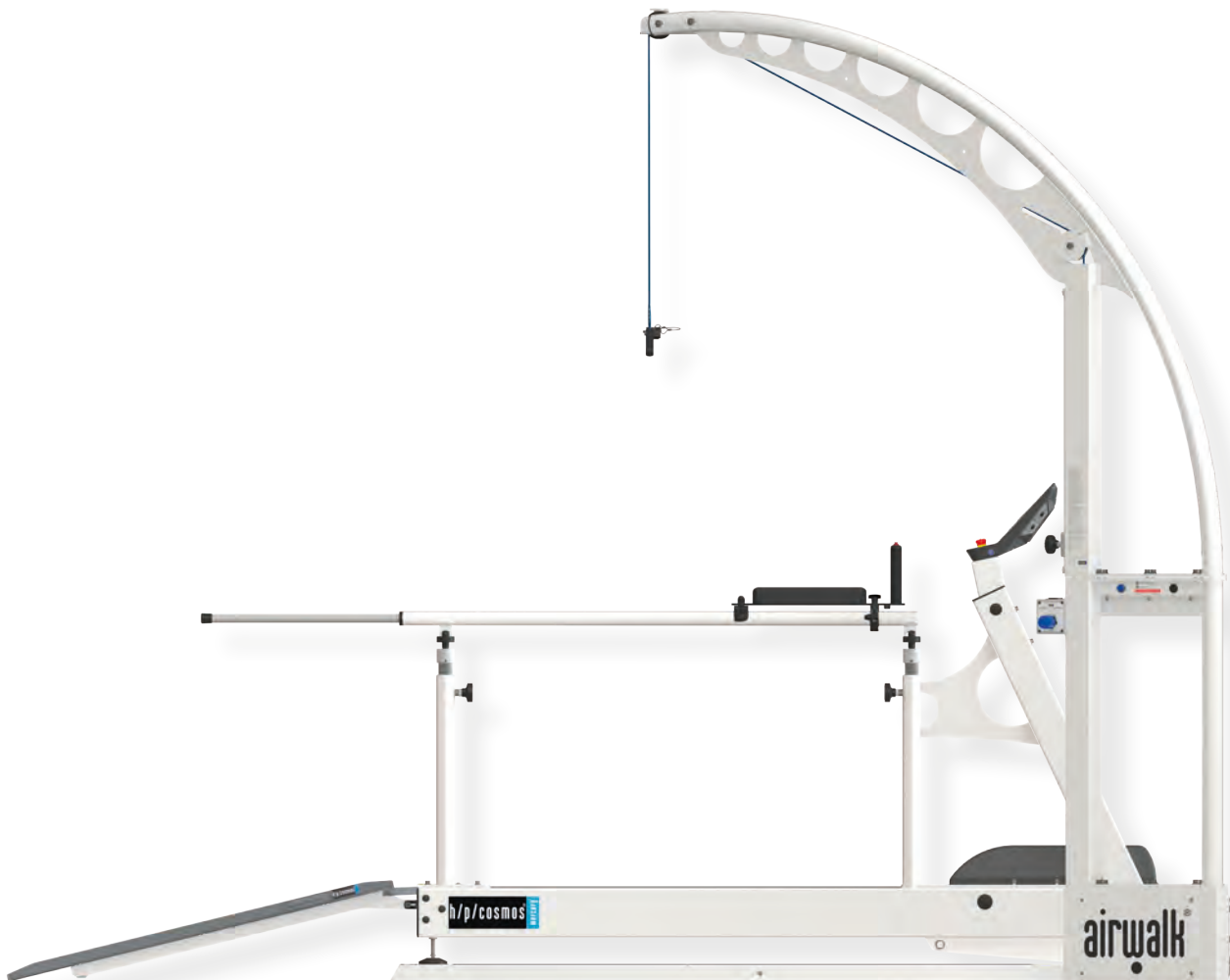
pluto® med with optional adjustable handrails [cos102010-01va01], airwalk® ap [cos30028] and wheelchair ramp [cos16186-02]
